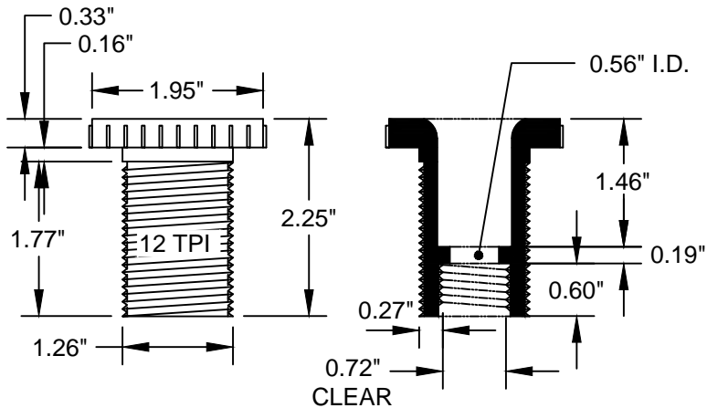
FRONT
